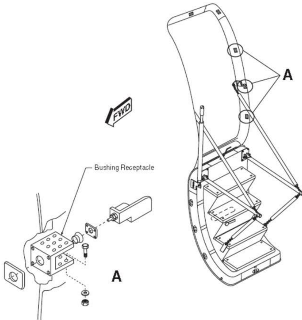
Figure 3H Click-Clack Bushing Receptacle
